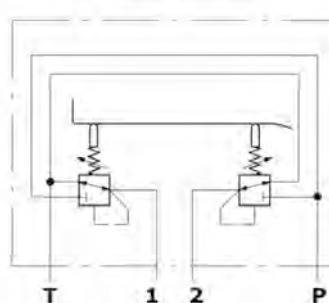
SVM500 Hydraulic circuit
