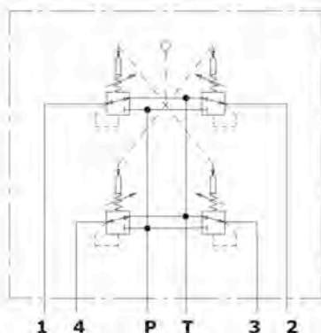
Hydraulic circuit
